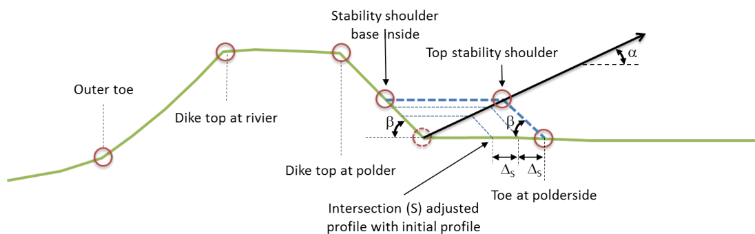
Figure E.7: Iterative shoulder development for macrostability
