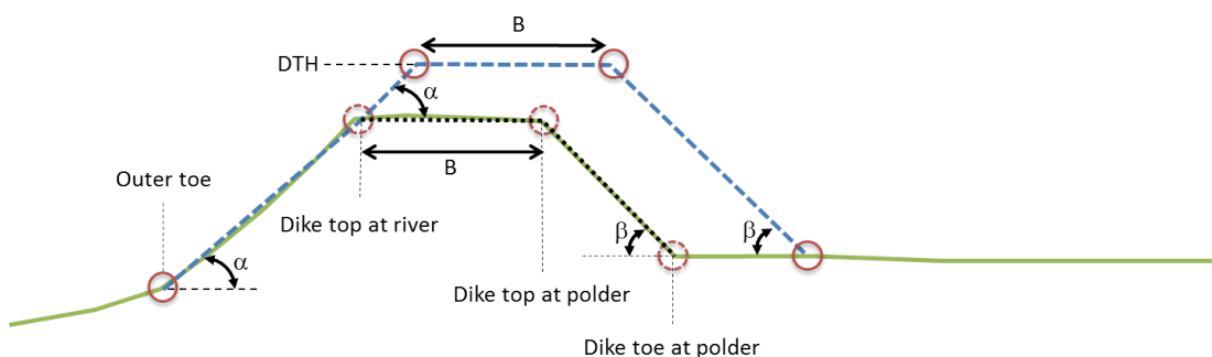
Figure E.1: Adapted geometry for DTH
