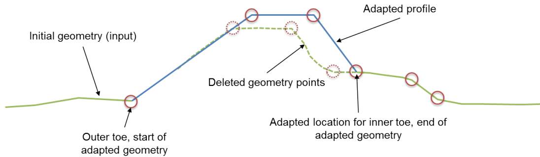
Figure E.2: Adapted geometry by deleting geometry points
