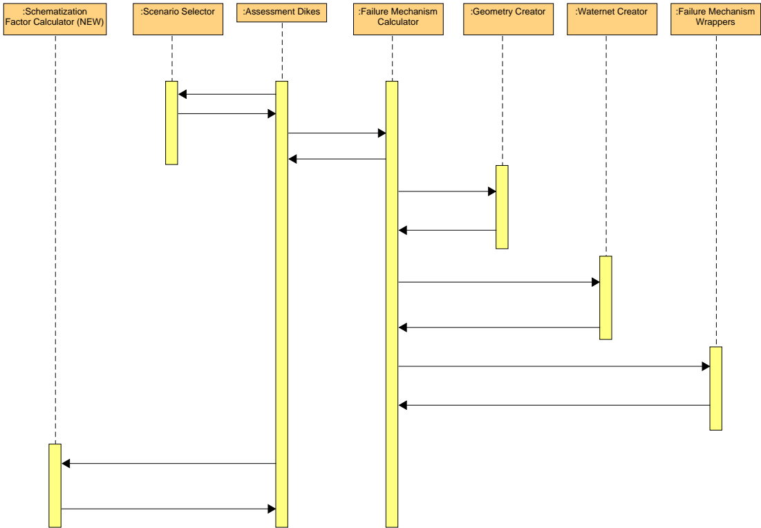
Figure 2.6: DAM Engine Regional assessment sequence diagram.
